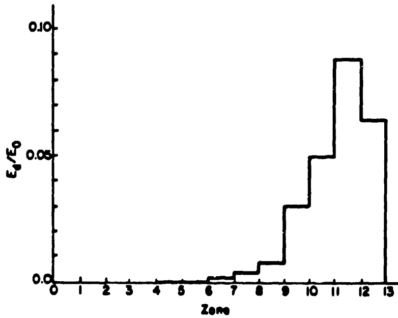
Fig. 12.--Fraction of initial proton energy deposited per zone to electrons for a beam entering at zone 13
