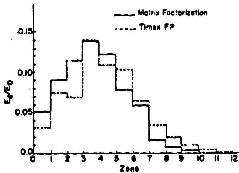
Fig. 3.--Fraction of initial alpha particle energy deposited per zone to ions
